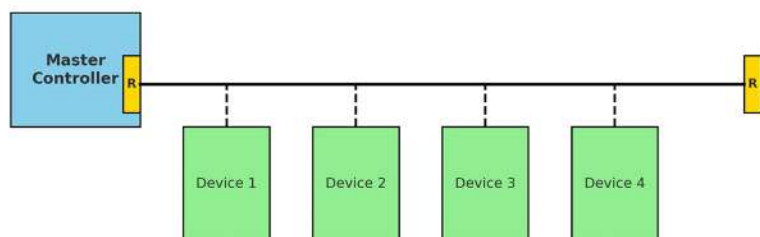
RS-485 System Architecture
